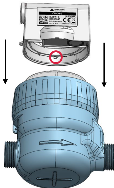
Fig. 7. View of the OP-O4-2 module, before mounting on the SV-RTK water meter.
