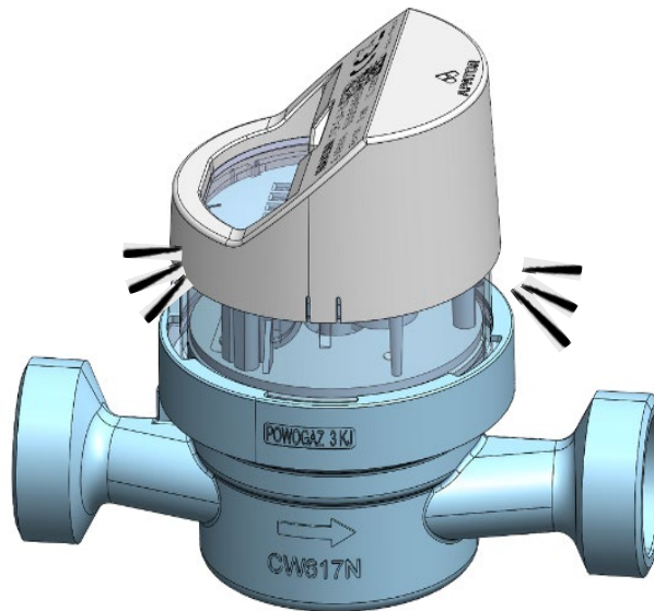
Fig. 6. View of the assembled JS Smart + water meter with the OP-O4-1b module.
